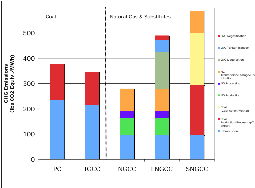
Figure 3: Midpoint Life Cycle GHG Emissions Using Advanced Technologies with CCS
